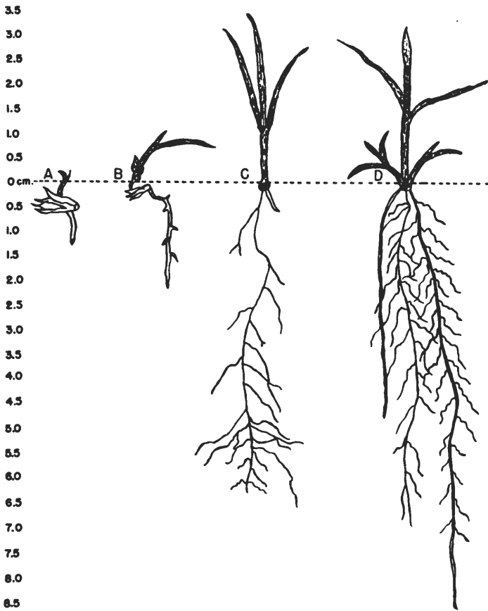
FIGURE 5. Stages in growth of blue grama seedling after emergence: (A) 24 hours. (B) One week. (C) Two weeks. (D) Three weeks.
