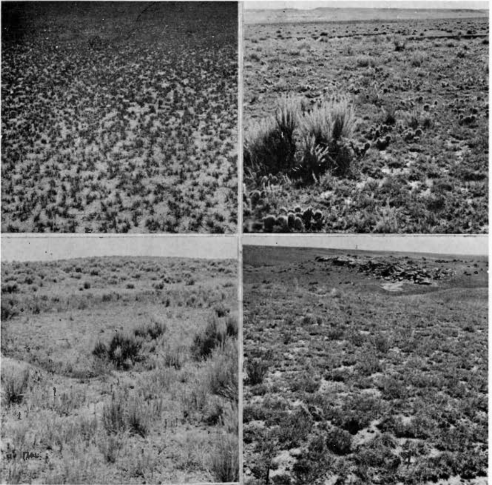
FIGURE 4. Four areas where blue grama forms an important part of the cover: (Upper left) On tight soil near Eads, Colorado. (Lower left) On dune sand at Woodward, Oklahoma, where sand sage forms a discontinuous upper story to the blue grama. (Upper right) On sandy loam north of New Raymer, Colorado. (Lower right) Blue grama on shallow soil above Foxhill Sandstone in Northeast Colorado.
