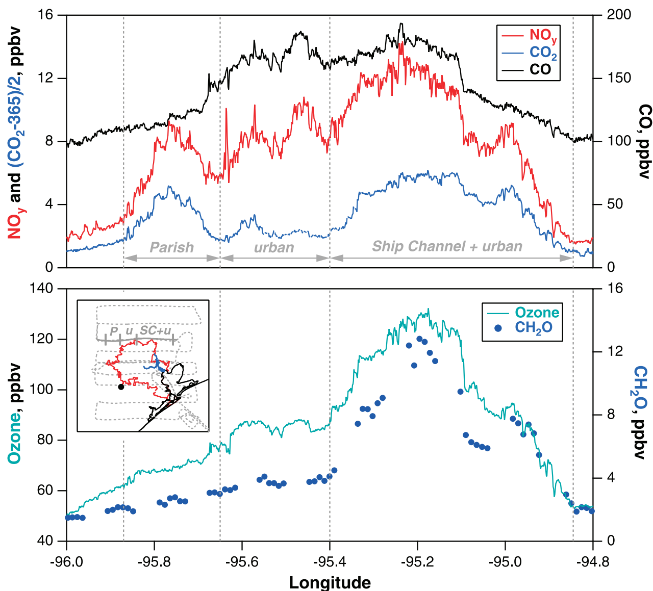
Figure 9. The inset map shows the E-W transect at 30.1° latitude on 28 August 2000 (solid gray line) along the aircraft flight track (dotted gray line). Locations of plumes from the W.A. Parish power plant “P,” the Houston urban core “u,” and the combined Ship Channel and urban plume “SC + u” along this transect are indicated by the vertical lines in the inset map and in the time series.
